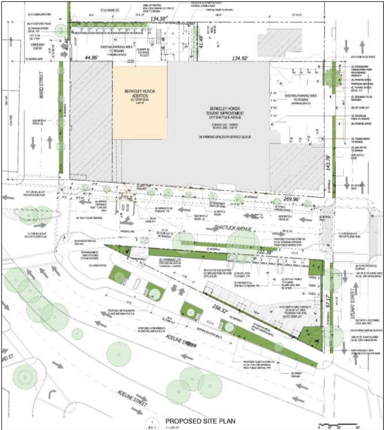
Figure 2: Proposed Site Plan 2777 Shattuck Avenue & 2747 Adeline Street
