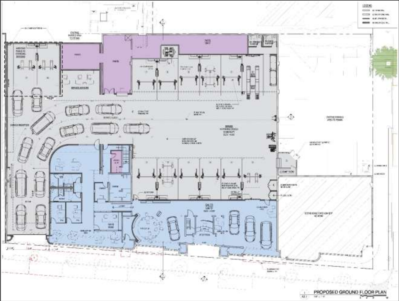
Figure 3: Proposed Ground Floor Plan – 2777 Shattuck Avenue
