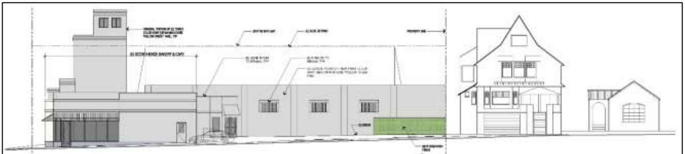
Figure 5: Proposed South Elevation
