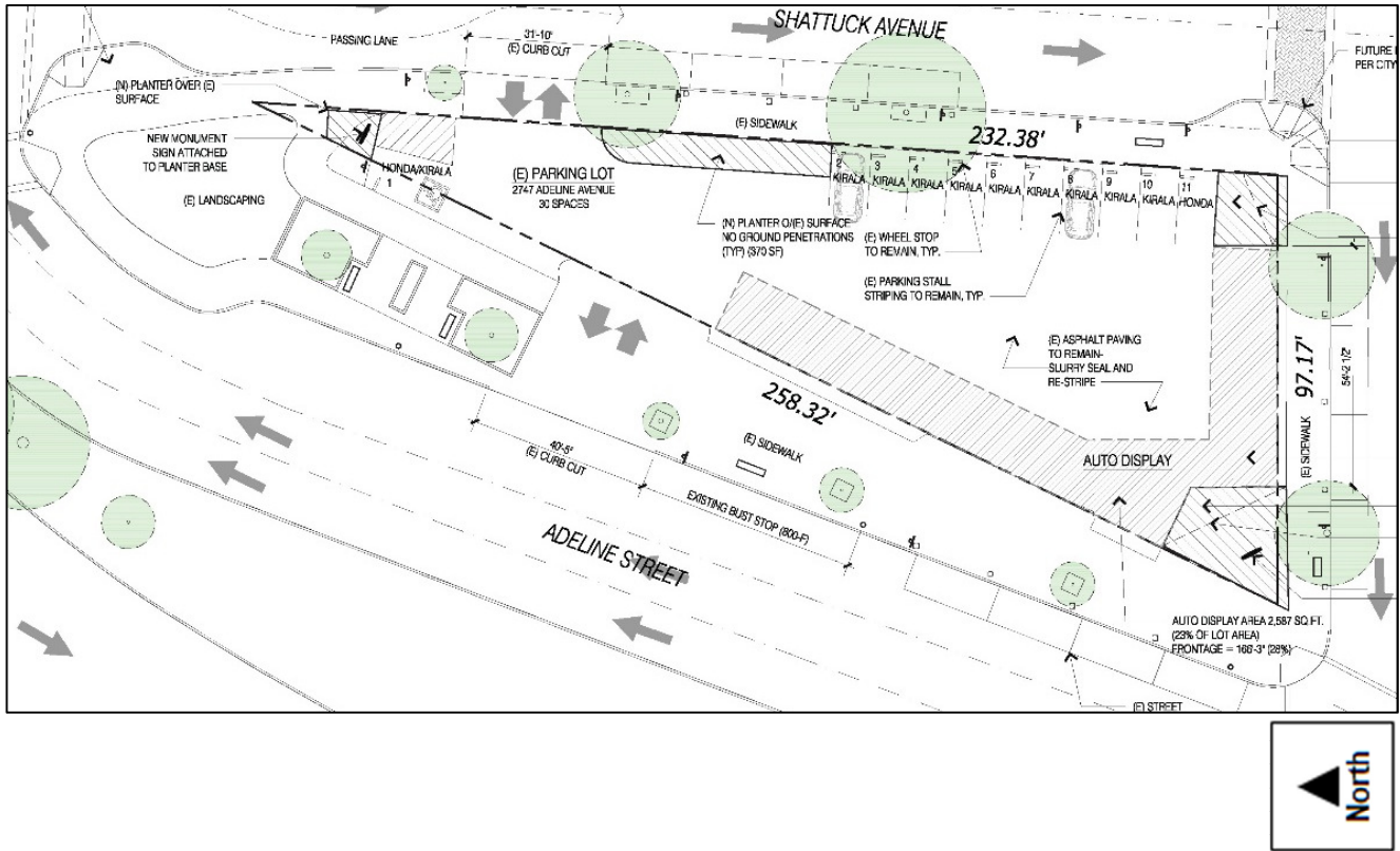
Figure 3: 2747 Adeline Street Site Plan
