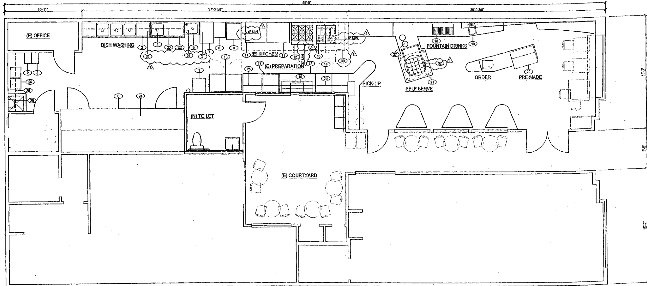
FOOD SERVICE EQUIPMENT PLAN
