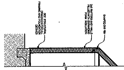
2 CROSS SECTION THROUGH HIGH CEILING, FINISHING DETAIL Scale: 1/4" = 1'-0"
