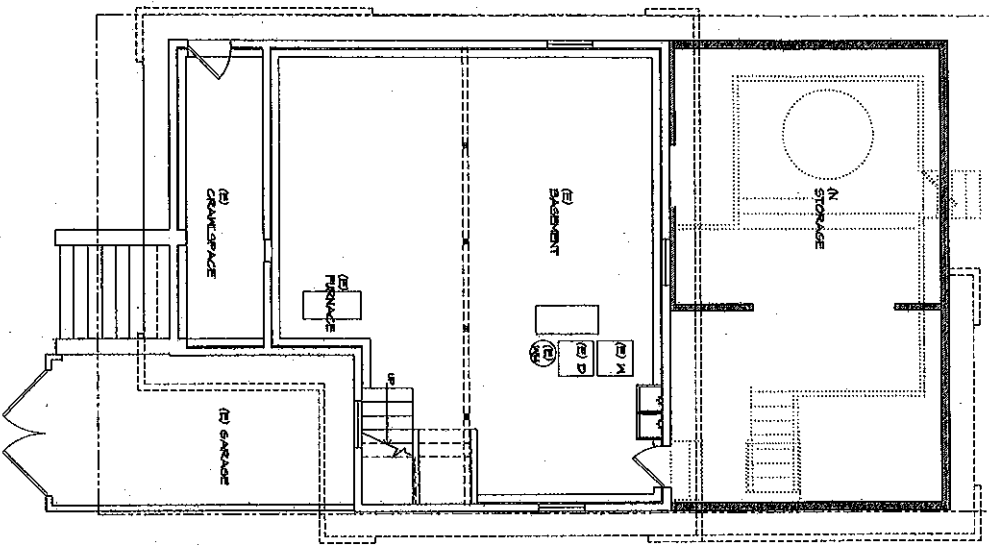
3 PROPOSED BASEMENT LEVEL FLOOR PLAN 1/4"=1'-0"
