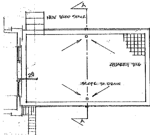
PROPOSED GARAGE ROOF PLAN 1/4" = 1'-0"
