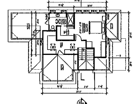
208 PROPOSED 3RD FLR PLAN
