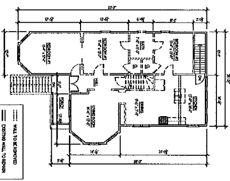
206 EXISTING/DEMO 2ND FLR PLAN
