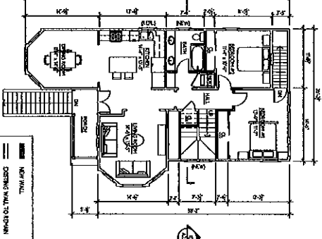
209 PROPOSED 2ND FLR PLAN
