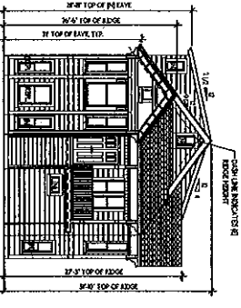
204 FRONT (SOUTH) ELEVATION
