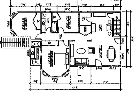
210 PROPOSED 1ST FLR PLAN
