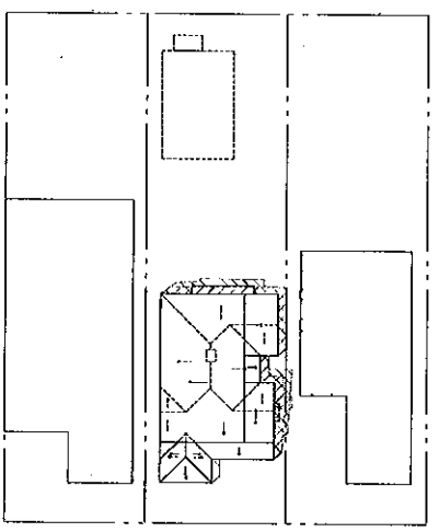
JUNE 21 - NOON
