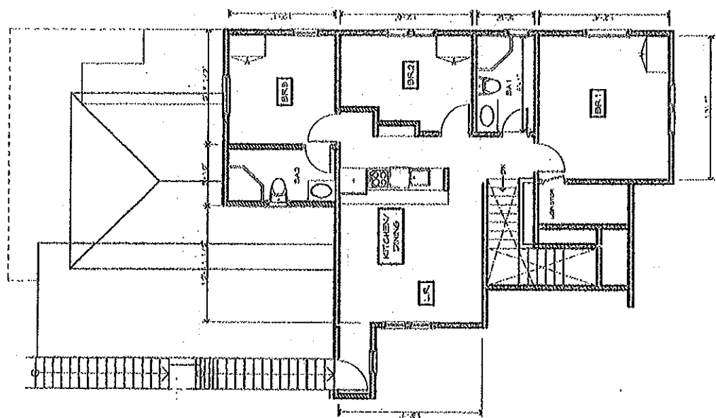
THIRD FLOOR PLAN SCALE 1/8" = 1'-0"
